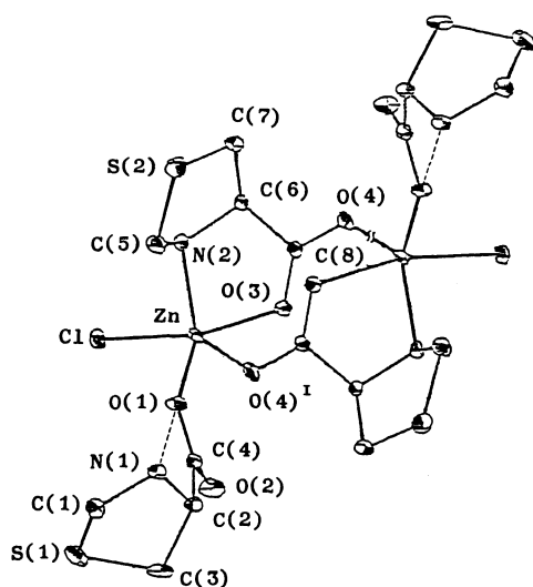
Fig. 1. The perspective drawing of \text{ZnClL(HL)} (zinc(II)-B) and the numbering scheme of non-hydrogen atoms.
