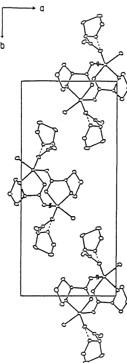
Fig. 2. The molecular packing of \text{ZnClL(HL)} (zinc(II)-B) along the c axis. -----: Hydrogen bonding.
